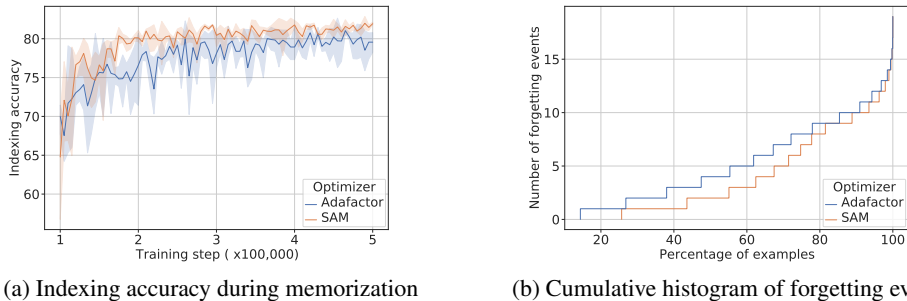
Figure 3: Investigating the effectiveness of SAM for alleviating implicit forgetting in the T5-Base model. (a) We observe serious fluctuations in the indexing accuracy in the case of the Adafactor optimizer, thereby, suggesting unstable memorization. SAM leads to relatively stable memorization of the documents. (b) A forgetting event (Toneva et al., 2019) is defined when an individual document goes from being classified correctly to incorrectly over the course of memorization. SAM increases the percentage of examples experiencing zero forgetting events by absolute 12% over Adafactor.
