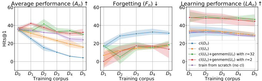
Figure 6: Investigating the effectiveness of generative memory in mitigating forgetting when continuously indexing new corpus D_n (T5-Base model and atomic docids representation) for the NQ dataset. \uparrow indicates higher is better, \downarrow indicates lower is better. We observe that continual indexing of old and new documents cl(U_n) help to alleviate forgetting of older documents when evaluated on retrieval tasks. However, average Hits@1 ( A_n ) still undergo 19 points drop after sequential updates ( D_0 \rightarrow D_1 \cdots \rightarrow D_5 ). We observe that by augmenting generative memory during continual indexing not only reduces the forgetting ( F_n ) but also improves average Hits@1 ( A_n ) by +17.3% over continual indexing.
