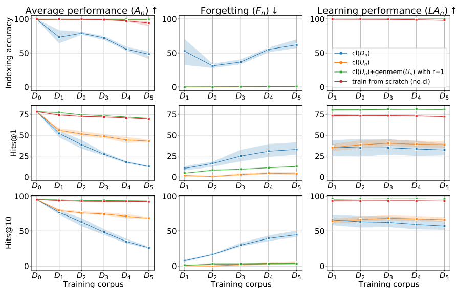
Figure 7: Investigating the effectiveness of generative memory in mitigating forgetting when continuously indexing new corpus D_n (T5-Base model and atomic docids representation) for the MS MARCO dataset. \uparrow indicates higher is better, \downarrow indicates lower is better. We observe that continual indexing of old and new documents cl(U_n) helps to alleviate forgetting of older documents when evaluated on retrieval tasks. However, average Hits@10 ( A_n ) still undergo 25.0 points drop after sequential updates ( D_0 \rightarrow D_1 \dots \rightarrow D_5 ). Generative memory enables sparse replaying of pseudo-queries for old documents and continual semi-supervised learning with new documents. We observe that augmenting generative memory during continual indexing not only reduces the forgetting ( F_n ) but also improves average Hits@10 ( A_n ) by +23.0% over considered baselines.
